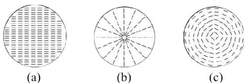
Fig 1. Liquid crystal configurations considered in this study: (a) uniform, (b) radial, and (c) circular.
